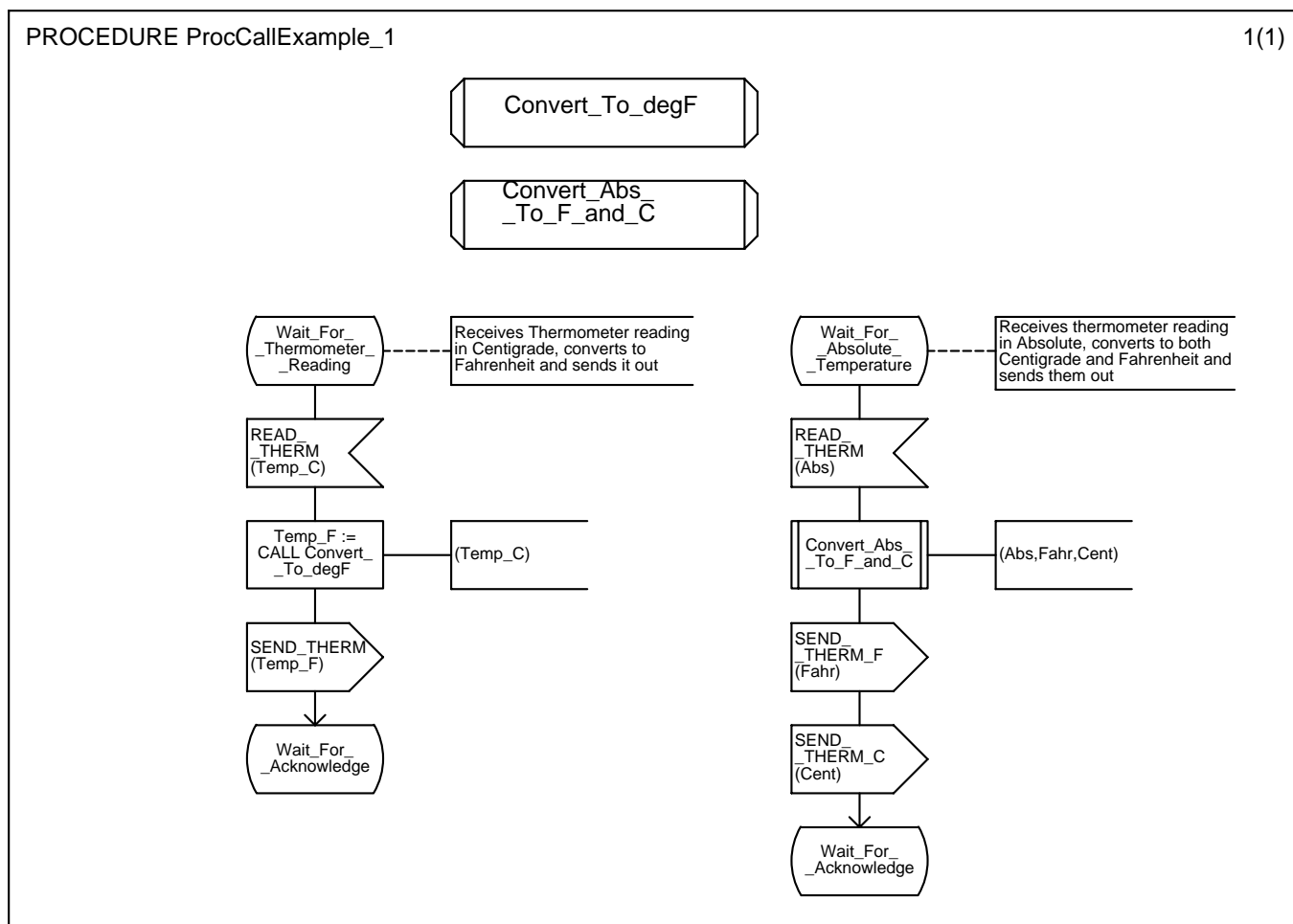
Figure 18: Examples of procedure calls
