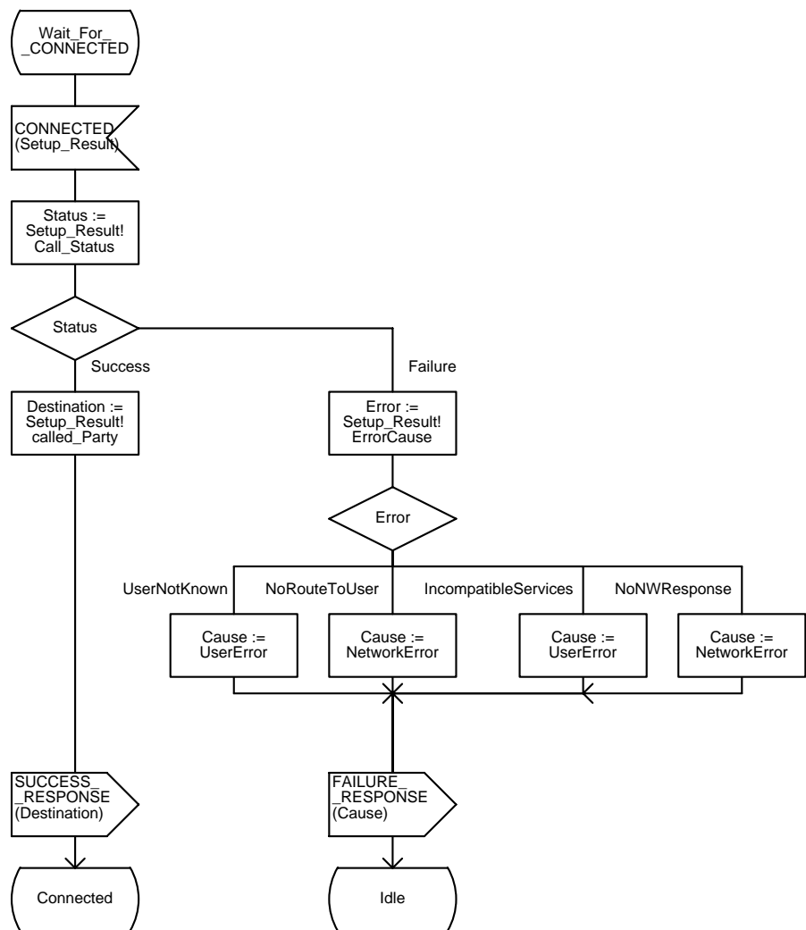
Figure 14: Message analysis example without the use of a procedure
