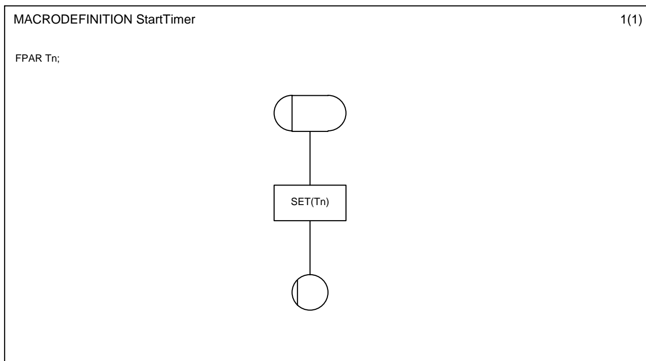
Figure 29: Macro definition for starting a timer
